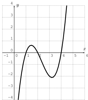
3 roots, 2 extrema
