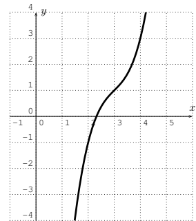
1 root, 0 extrema
