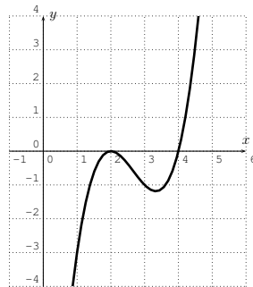
2 roots, 2 extrema
